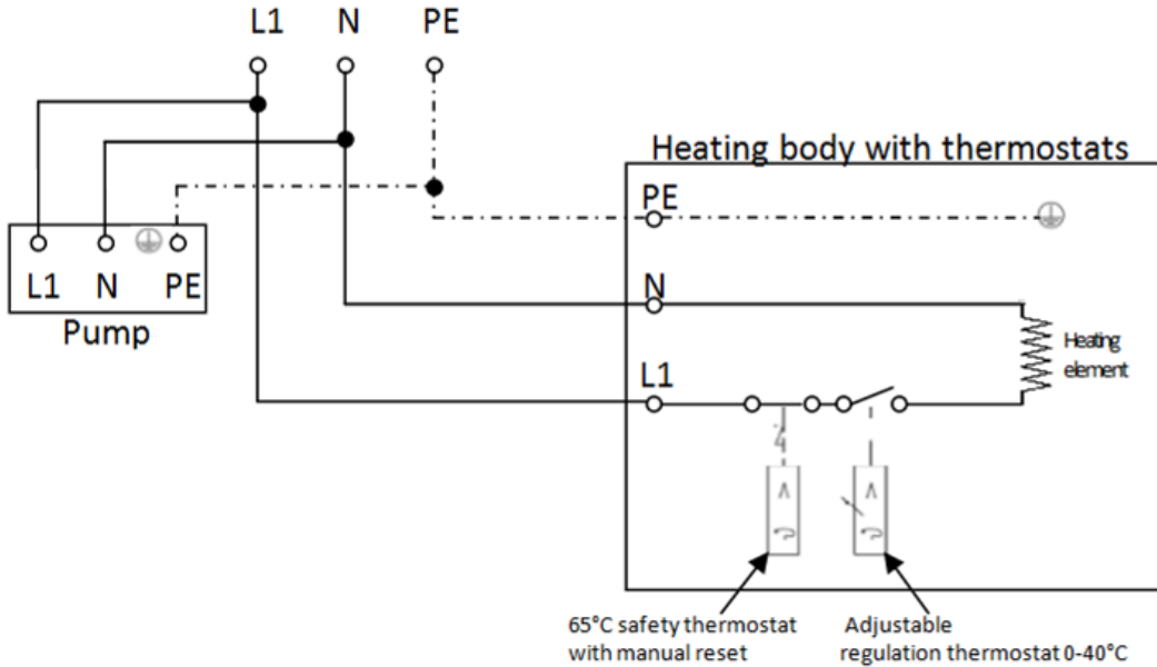
Aqualine without control box
