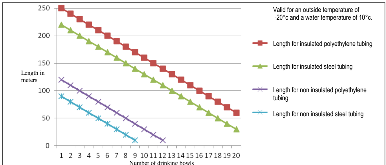
Diagram 1: Maximum length for 3/4" tubing or 20 mm inside diameter
