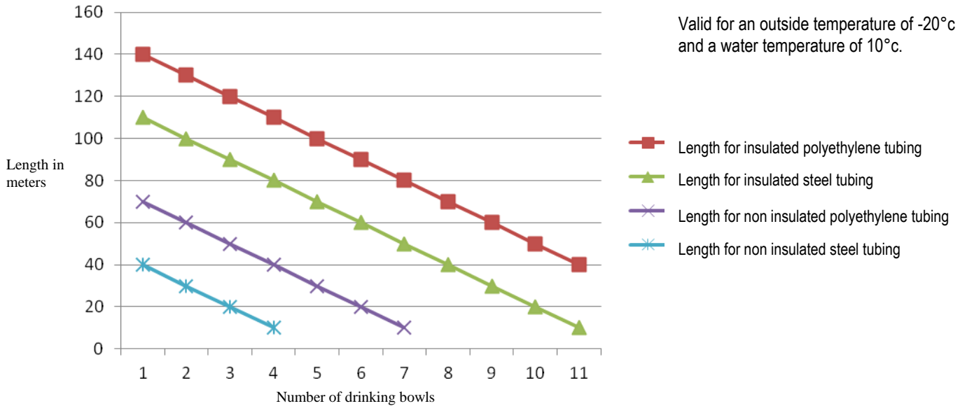
Diagram 2: Maximum length for 1/2" tubing or 15 mm inside diameter
