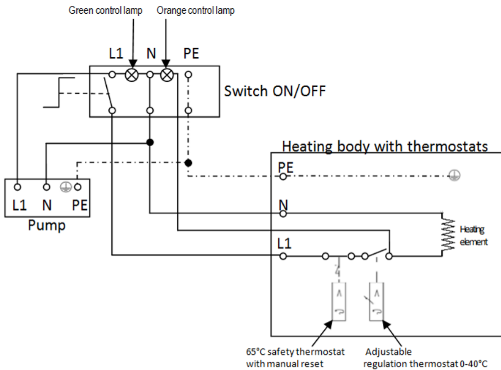
Aqualine with control box
