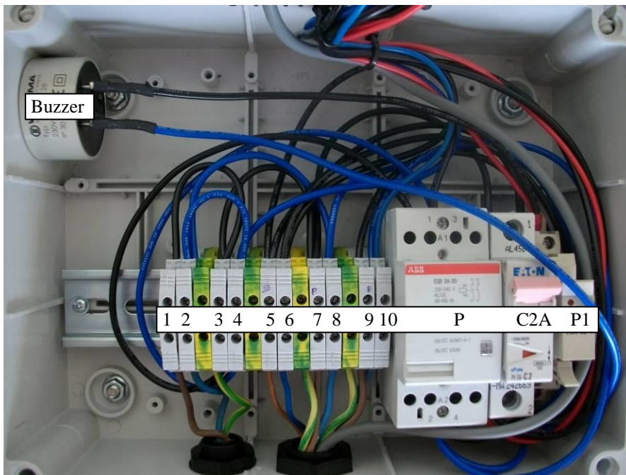
Picture inside digital control box
